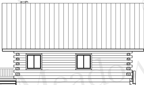
LEFT ELEVATION
