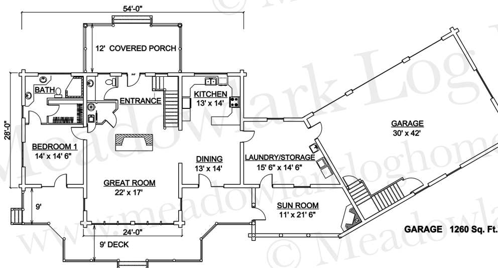
MAIN FLOOR 2372 Sq. Ft.
