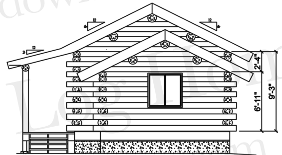
LEFT ELEVATION
