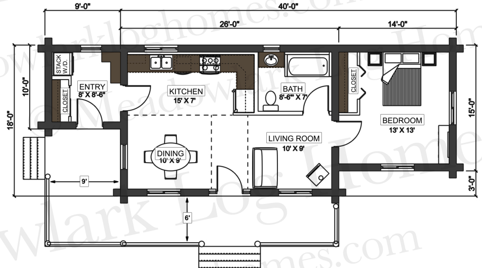
FLOOR PLAN
